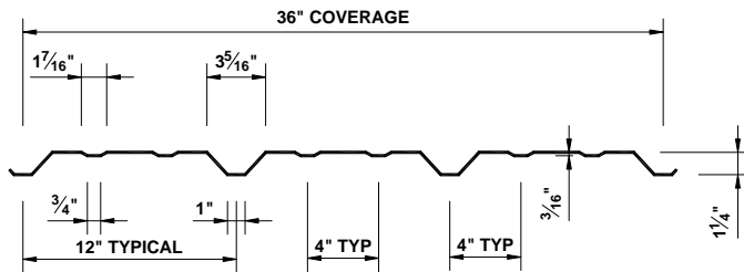
BIGBEE-RR Architectural Cross Section
